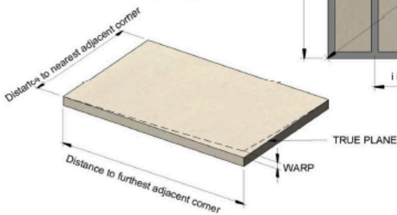
FIGURE 4 Warping
