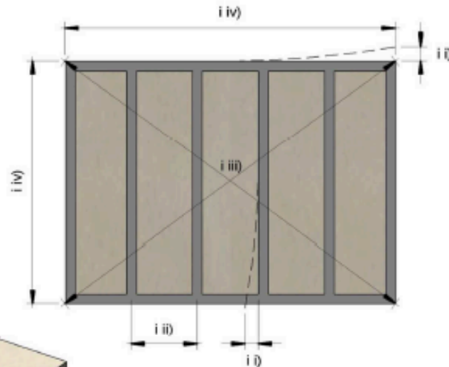
FIGURE 3 Stud Frame
